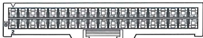
2*19P
