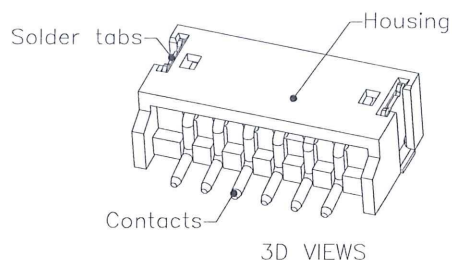
Assembly Layout
