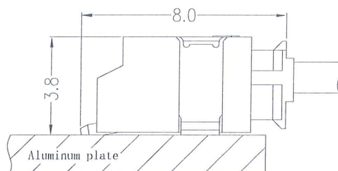
Assembly Layout
